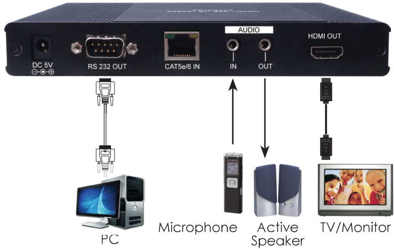
Receiver's Rear Panel
